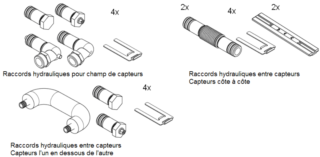
Figure 5 – Raccords hydrauliques.
